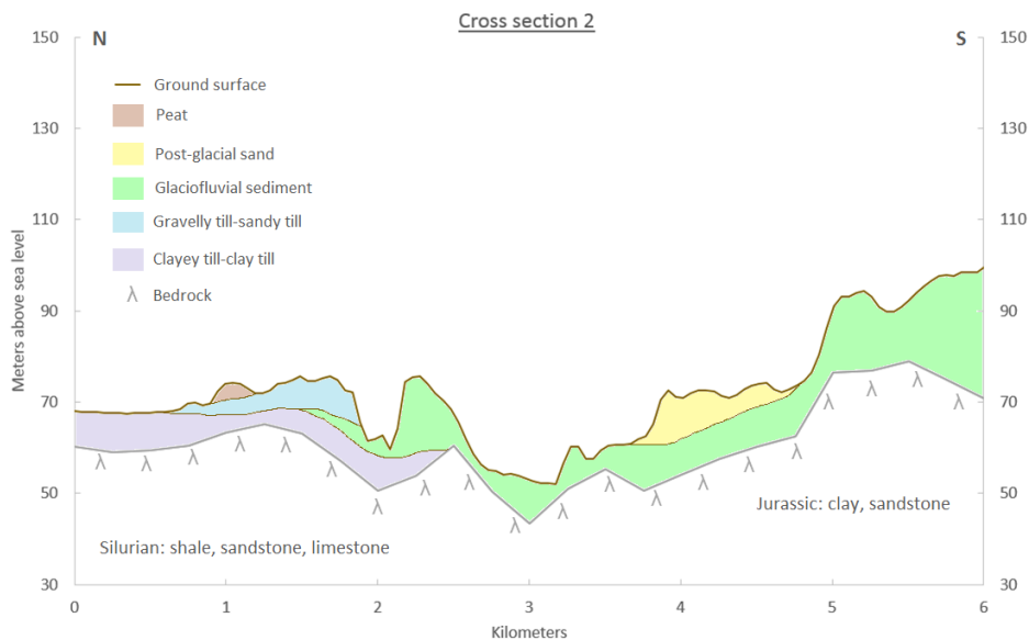
Figure 2.11: Section 2: Cross section from north to south over the Vomb basin east of Sjöbo. Illustration produced in Excel and Paint by the authors.
